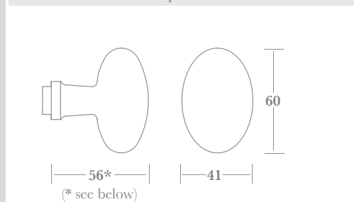
▲ 7621 with 6000B plate
