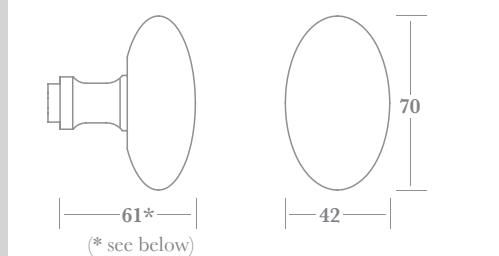
▲ 7616 with 6000B plate
