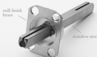
▲ 7806 Access Control (AC) Spindle
